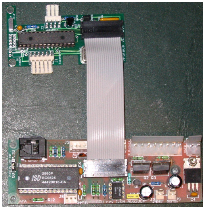
Figure 4. Proteus plugged into BFS board
